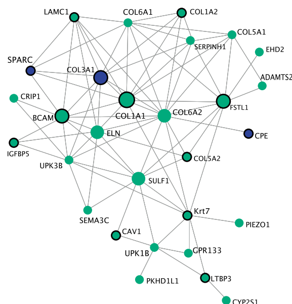
Figure 4. Visualization of the most connected genes in the female “royalblue” (A) and the male “black” (B) co-expression modules with VisANT (Hu et al. 2008). The royalblue module is associated with BMI ( P = 2 \times 10^{-8} ) and body length variation ( P = 6 \times 10^{-6} ). The black module is associated with BMI ( P = 5 \times 10^{-8} ), body mass ( P = 0.001 ), and body length variation ( P = 3 \times 10^{-10} ). Blue circles represent genes for which we identified a cis -eQTL that explains a component of expression variation. Circles with black borders are genes with mutant phenotypes related to body size or metabolism. Phenotype information was collected from MGI (Blake et al. 2017).
